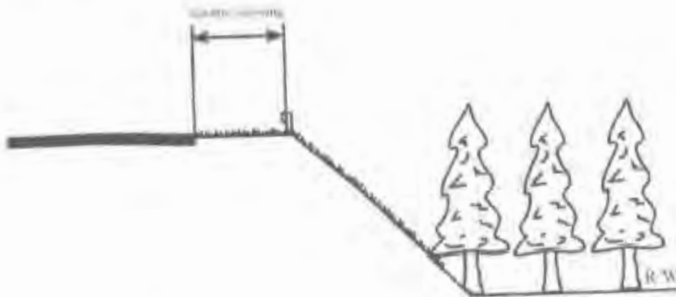
TYPICAL FILL SECTION WITH GUARDRAIL NEAR SHOULDER POINT For Swath and Ditch Contracts:
